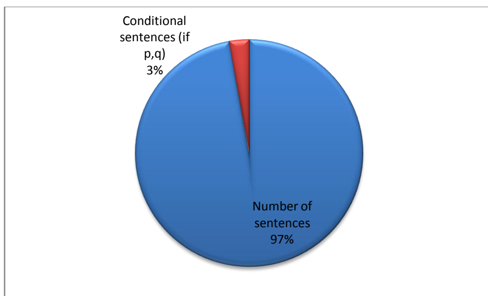
Chart 4 – Number of conditional sentences in the corpus
